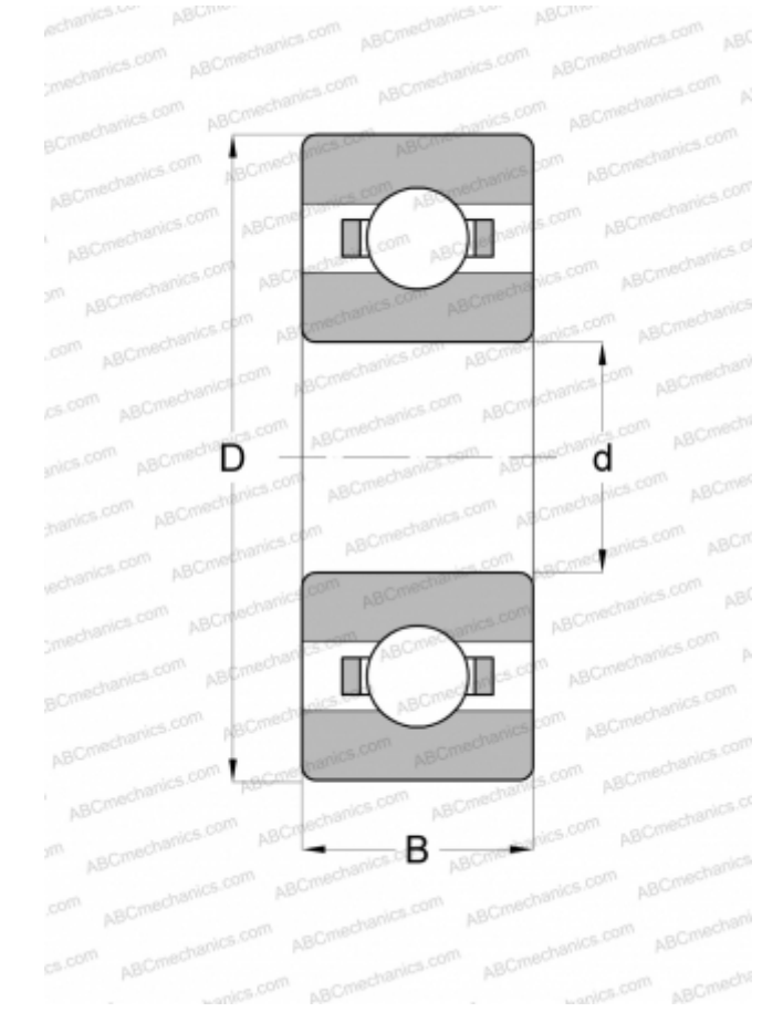
DIMENSIONS, MM
