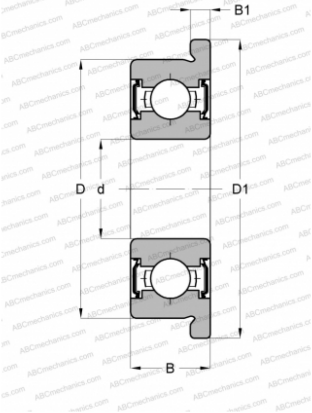
DIMENSIONS, MM
